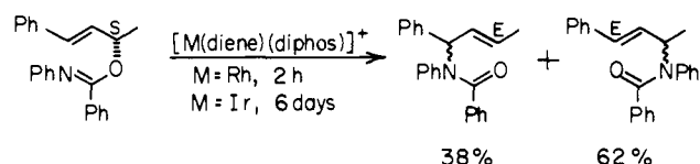
Figure 11. Rearrangement products which are formed by rhodium(I) and iridium(I) catalysis of the optically active allyl imidate.
