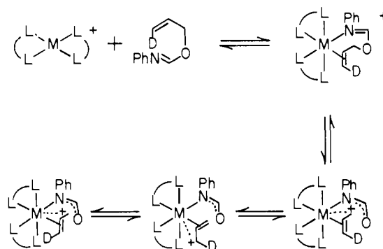
Figure 13. Proposed carbonium ion mechanism that could cause rearrangement of an allyl imidate. Shown is the fragmentation of an allyl imidate coordinated to either rhodium(I) or iridium(I). The mechanism for cis–trans olefin isomerism is shown as occurring via 1,3-carbonium ion shifts, a mechanism which also leads to loss of optical activity. The products are formed by combination of the carbonium ion with the coordinated nitrogen atom of the amide anion.
